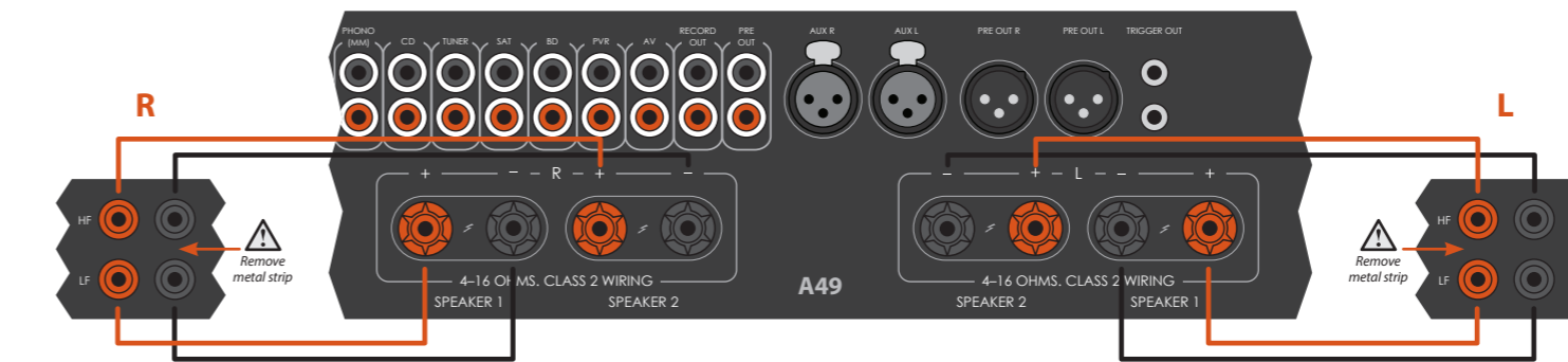
An A49 connected to two sets of speakers using bi-wiring.
